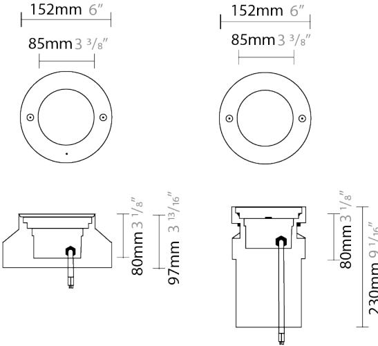
Housing L9A08800
